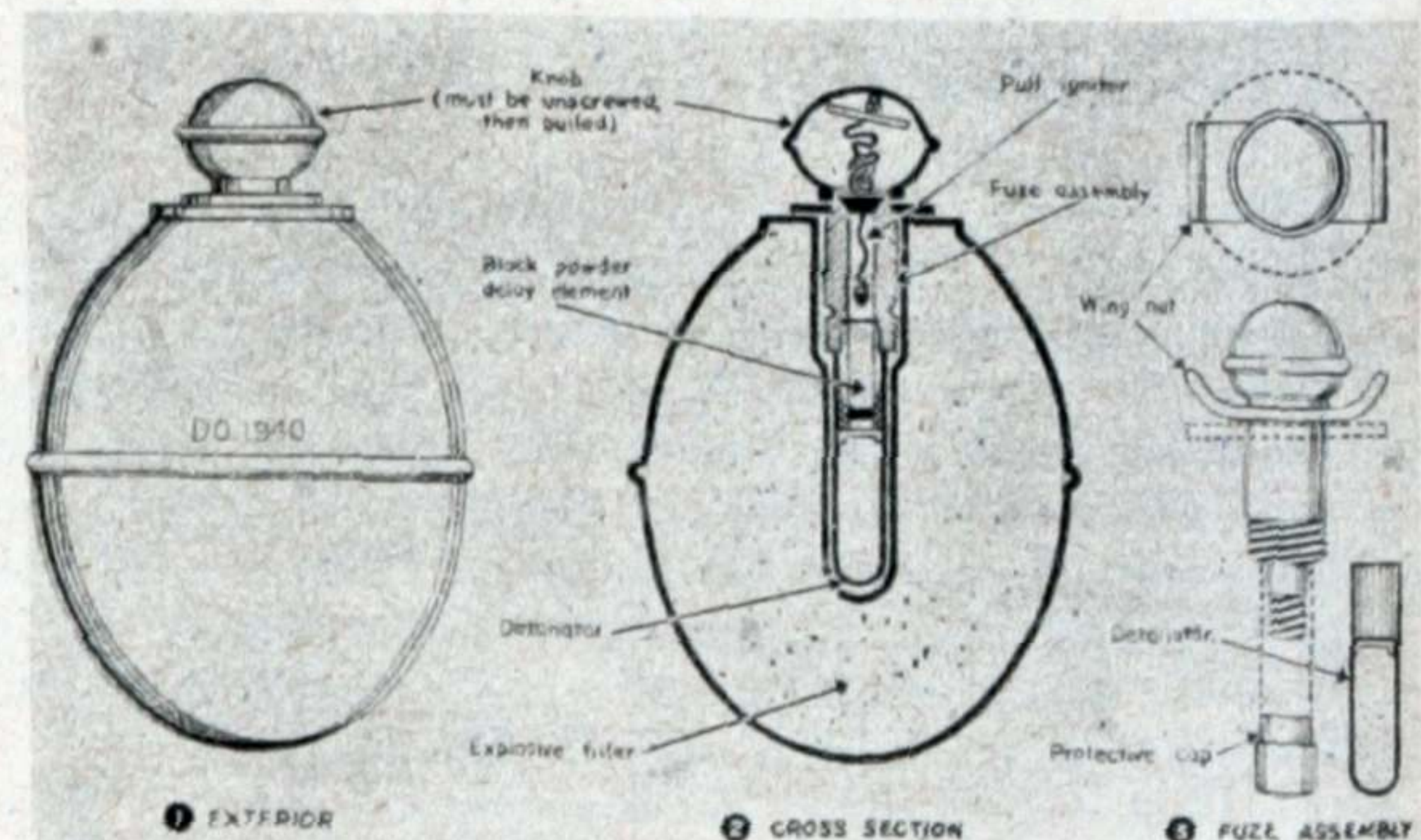
Sketch of egg-type hand grenade, Model 39.
